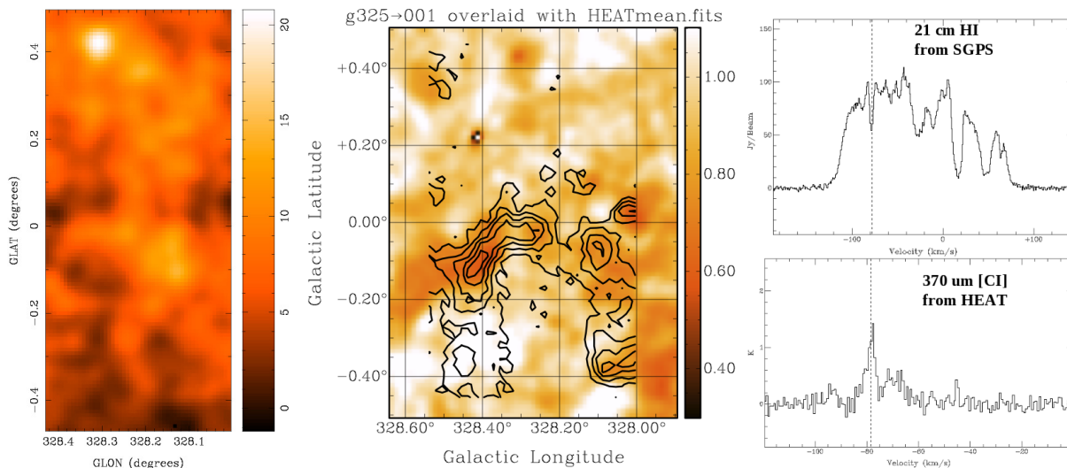
Figure 4: (left) Integrated intensity map of [CI] line emission toward l=328^\circ shows that diffuse atomic carbon emission fills the Galaxy and is nearly as abundant as CO. (center) The molecular gas shown by HEAT’s detected line emission at -78 \text{ km/s } V_{lsr} (contours) appears to be associated with self-absorption in the 21 cm HI line (color scale) at the same velocity. The high abundance of [CI] suggests that this molecular gas is chemically-young; it has not yet converted much of its elemental carbon to CO. Such a signature is indicative of a natal cloud. Establishing where these clouds are forming in a Galactic context is one of the primary goals of the HEAT telescope and one of the main motivations to extend its initial mission.
