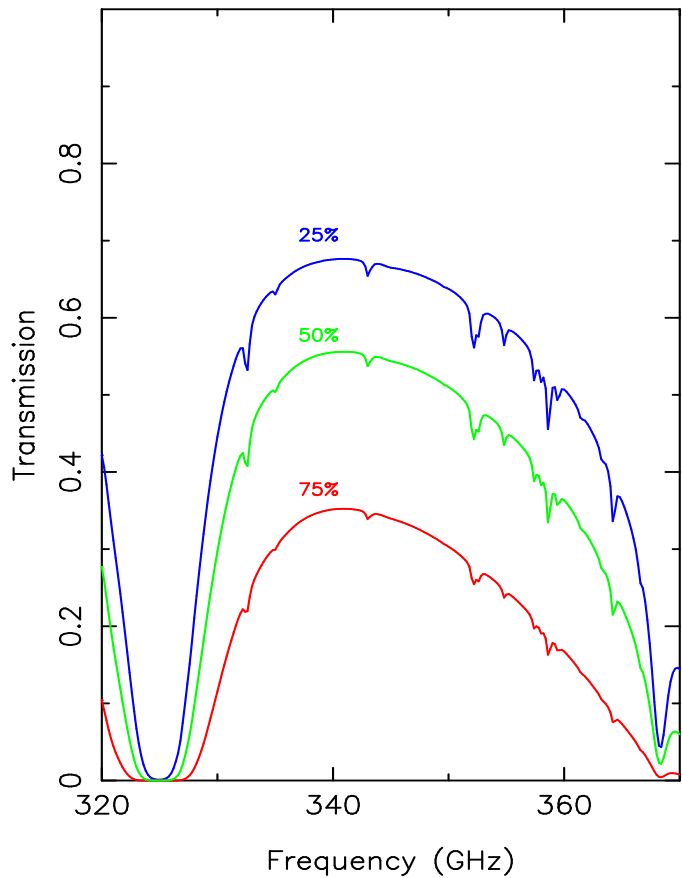
Atmospheric Transmission
