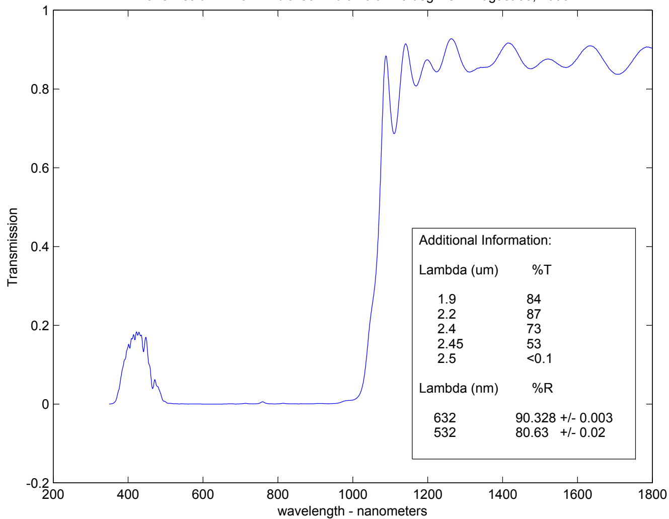
Transmission - 120 mm dia CaF2 dichroic - 15 deg AOI - August 03, 2006
