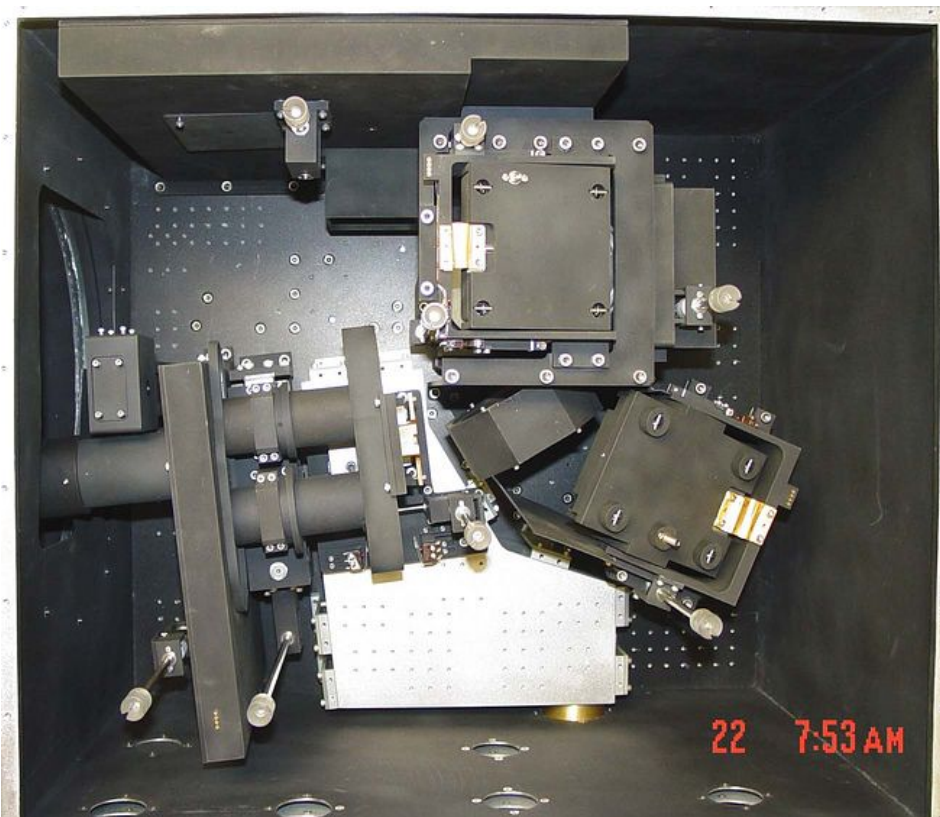
Photo of “empty” ARIES top spectrometer vessel
